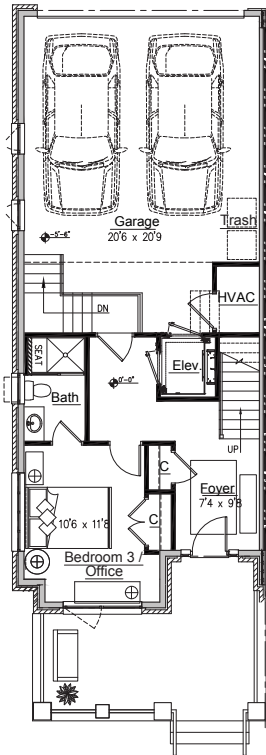
First Floor
