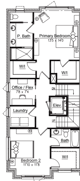
Third Floor
