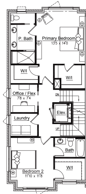
Third Floor
